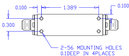
Dimensions in inches
